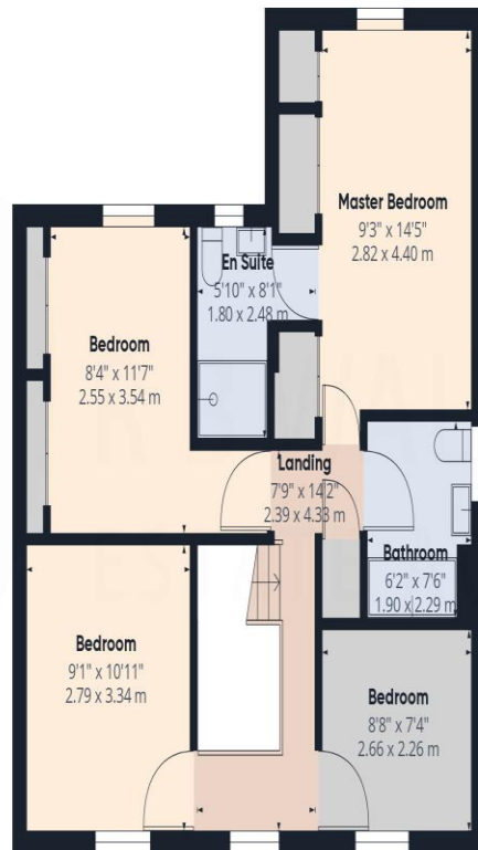
Floor 1 Building 1
