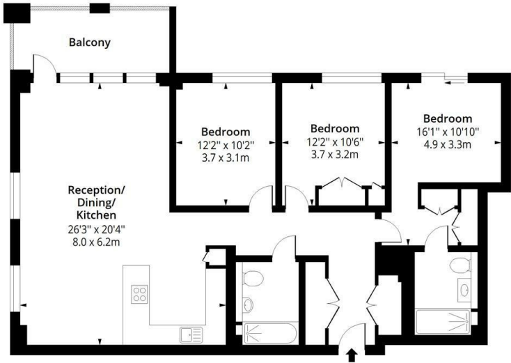
Tenth Floor Floor Area 1186 Sq Ft - 110.18 Sq M
