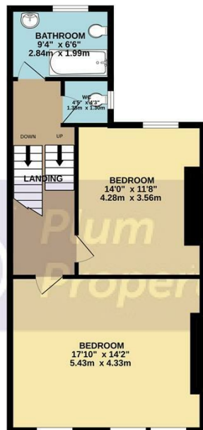
1ST FLOOR 588 sq.ft. (54.6 sq.m.) approx.
