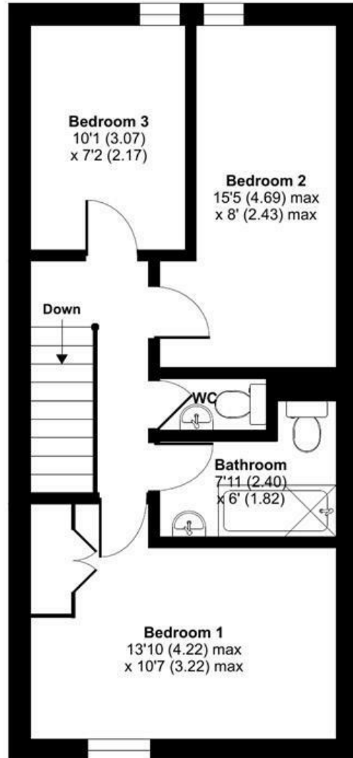
THIRD FLOOR
