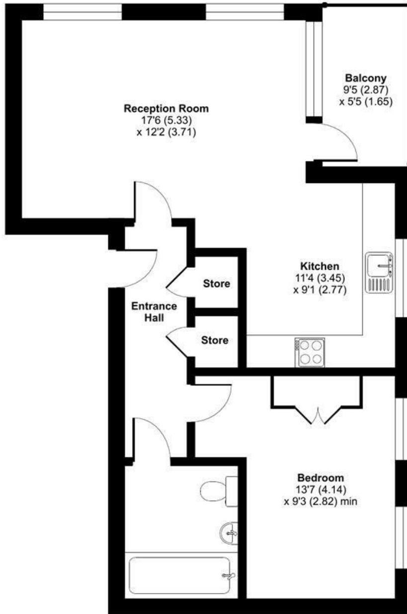
THIRD FLOOR
