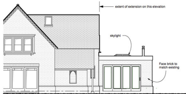
Extension South Elevation
