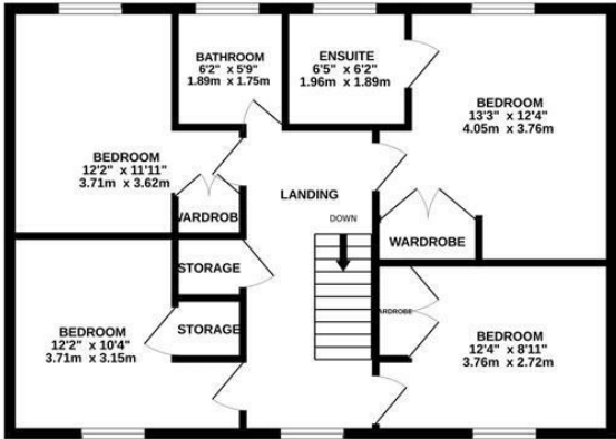
2ND FLOOR 699 sq.ft. (64.9 sq.m.) approx.
