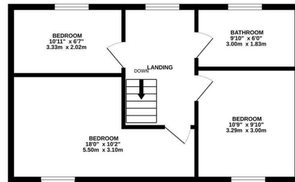
1ST FLOOR 467 sq.ft. (43.4 sq.m.) approx.
