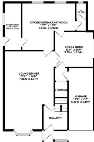
GROUND FLOOR 892 sq.ft. (82.9 sq.m.) approx.
