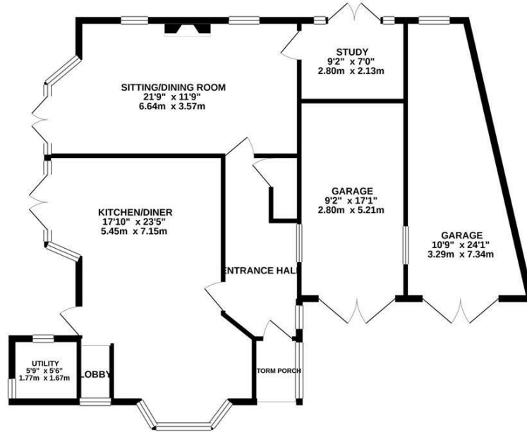
GROUND FLOOR 1128 sq.ft. (104.8 sq.m.) approx.
