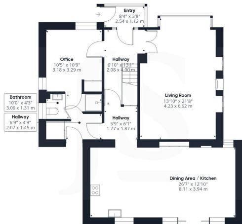
Floor 0 Building 1
