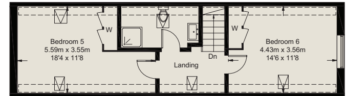
Second Floor 46.0 sq m / 495 sq ft
