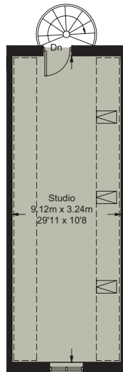
Outbuilding - First Floor 29.9 sq m / 322 sq ft
