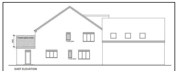
EAST ELEVATION
