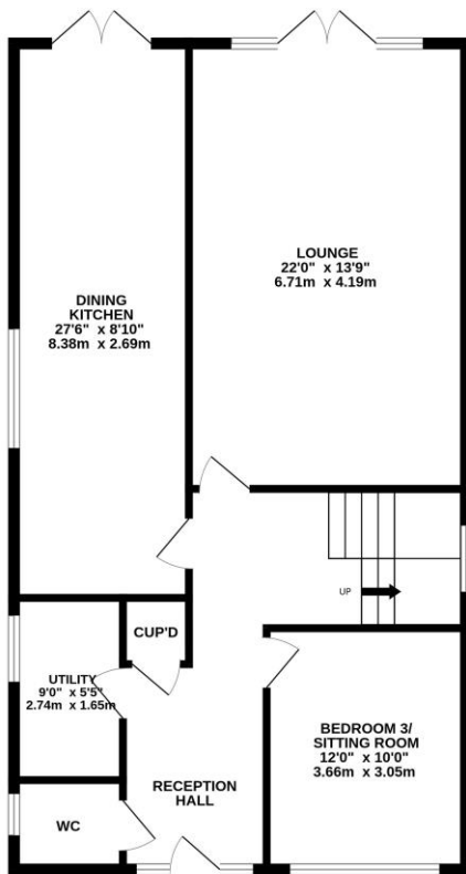
GROUND FLOOR 923 sq.ft. (85.8 sq.m.) approx.
