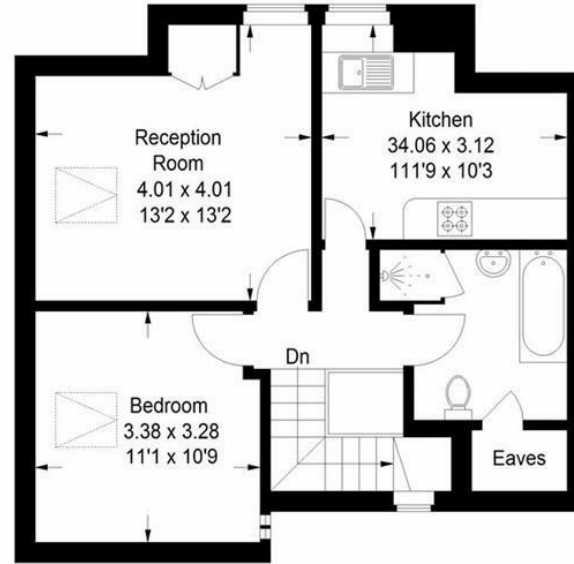
Second Floor
