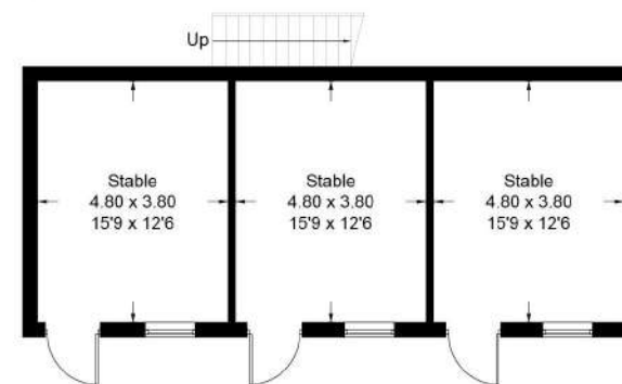
Stable - Ground Floor
