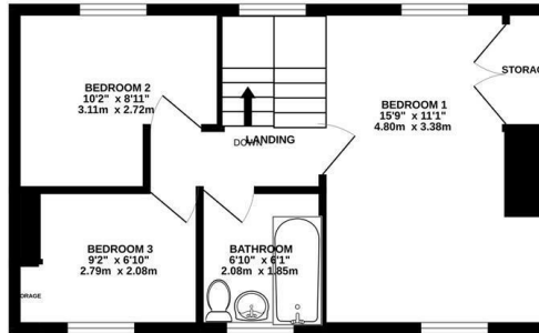
1ST FLOOR 403 sq.ft. (37.4 sq.m.) approx.
