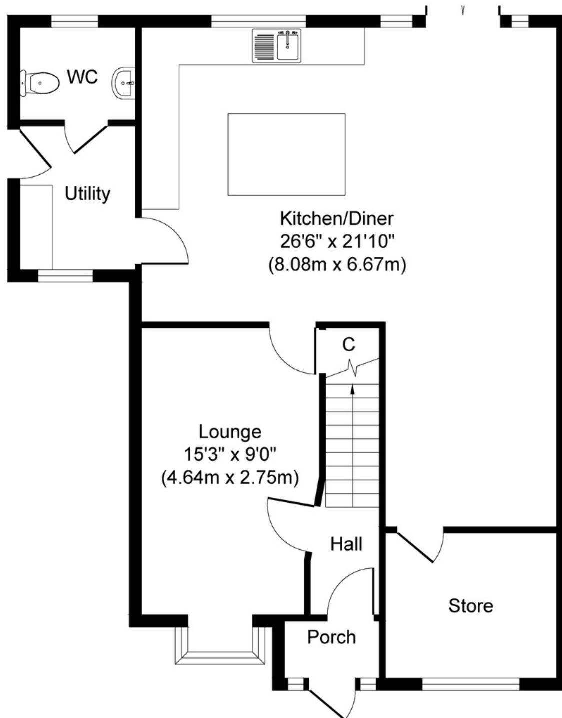
Ground Floor Approximate Floor Area 817 sq. ft
