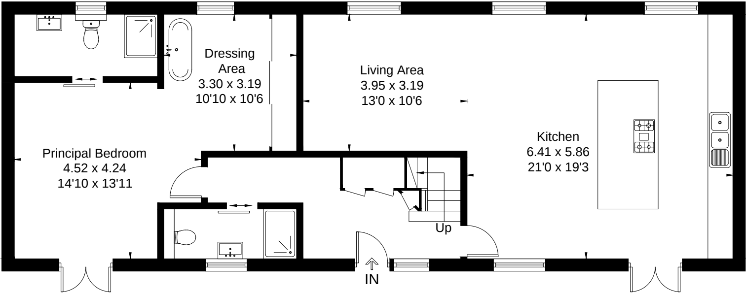
Ground Floor
