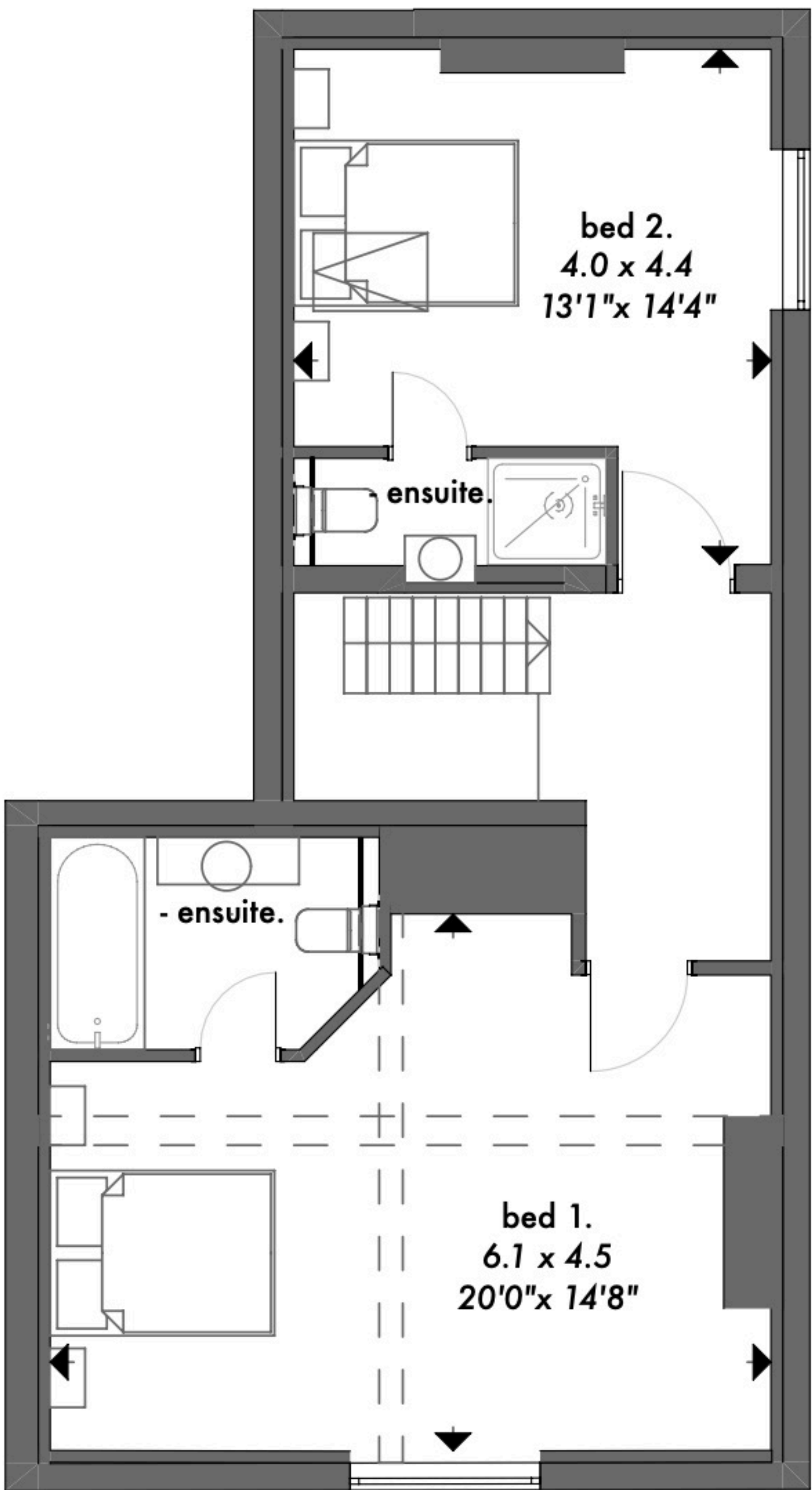
First Floor
