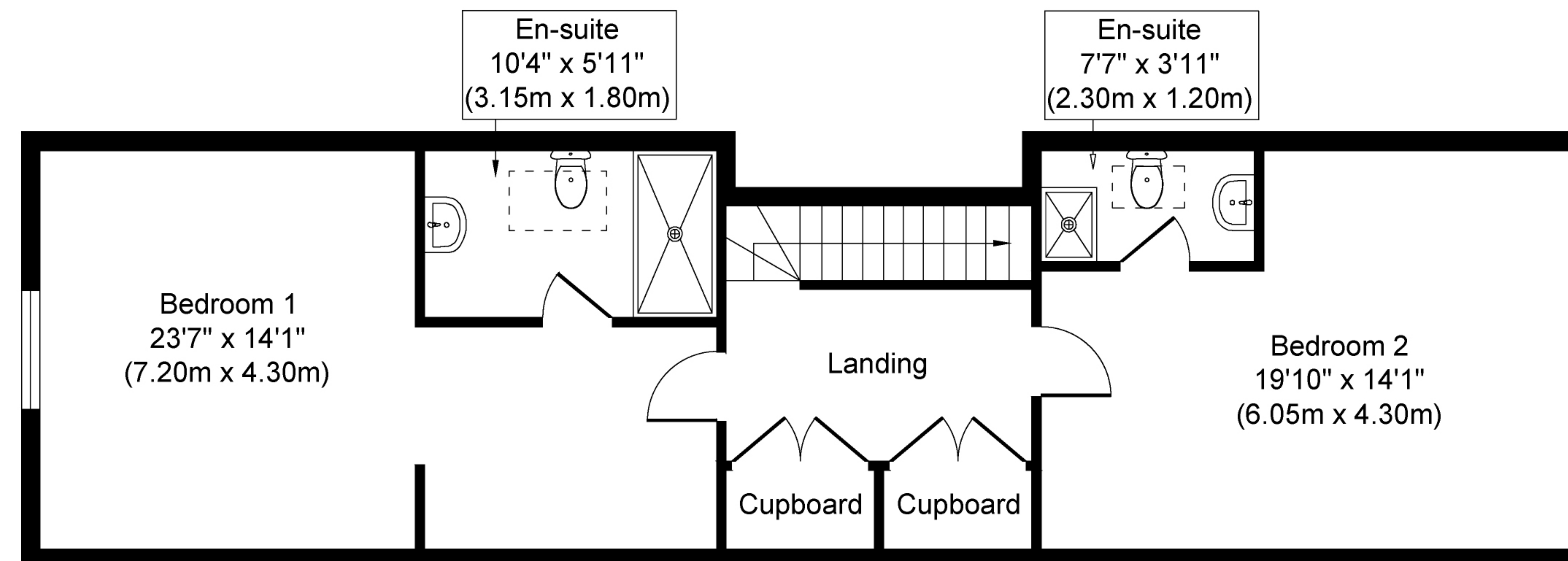
First Floor Approximate Floor Area 743 sq. ft (69.06 sq. m)
