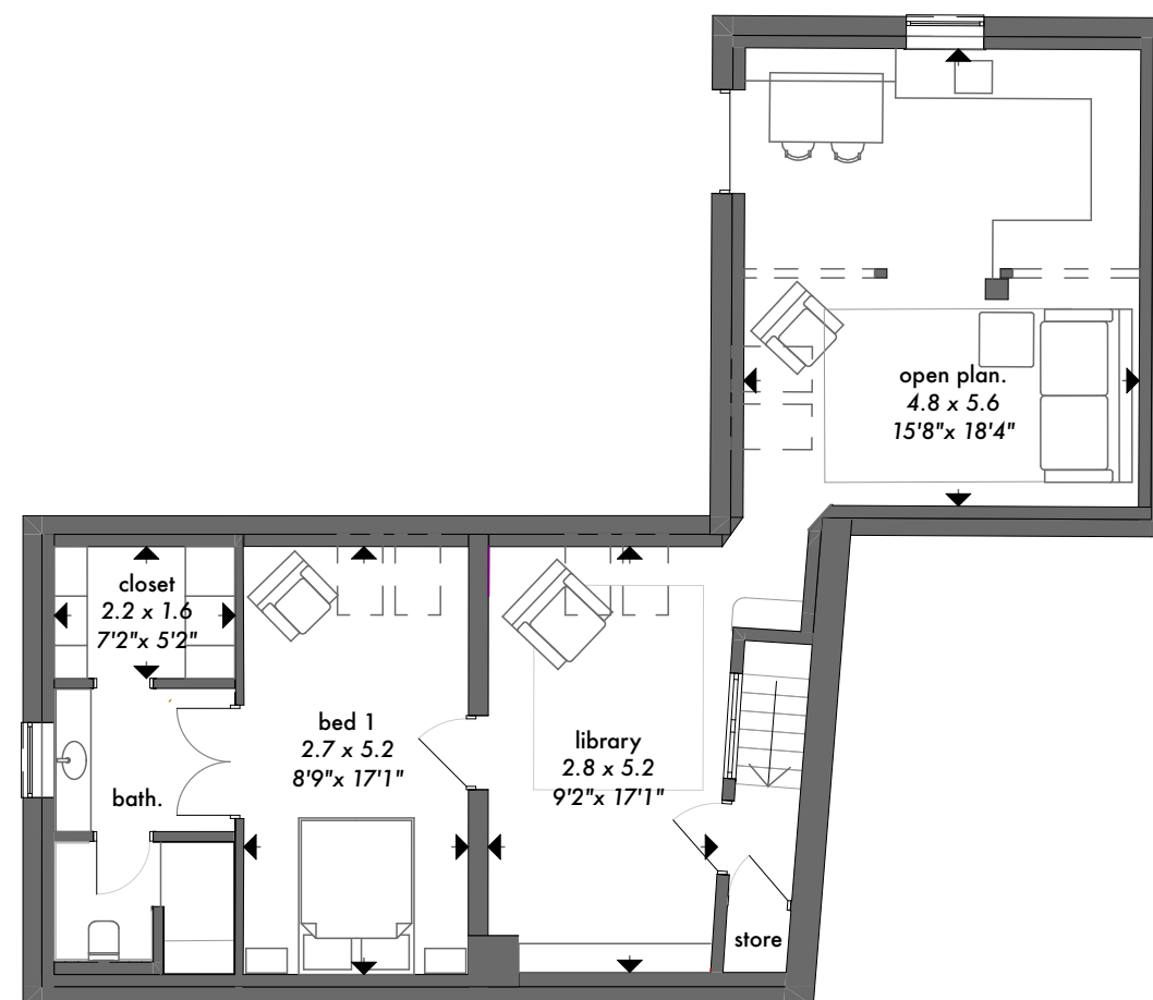
First Floor
