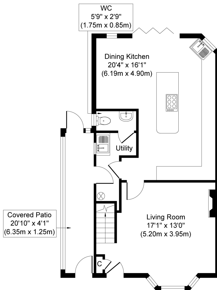
Ground Floor Approximate Floor Area 670 sq. ft (62.24 sq. m)
