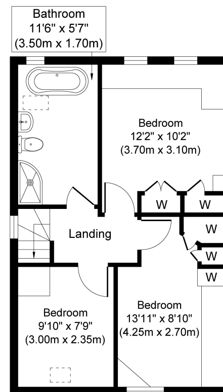
First Floor Approximate Floor Area 451 sq. ft (41.86 sq. m)
