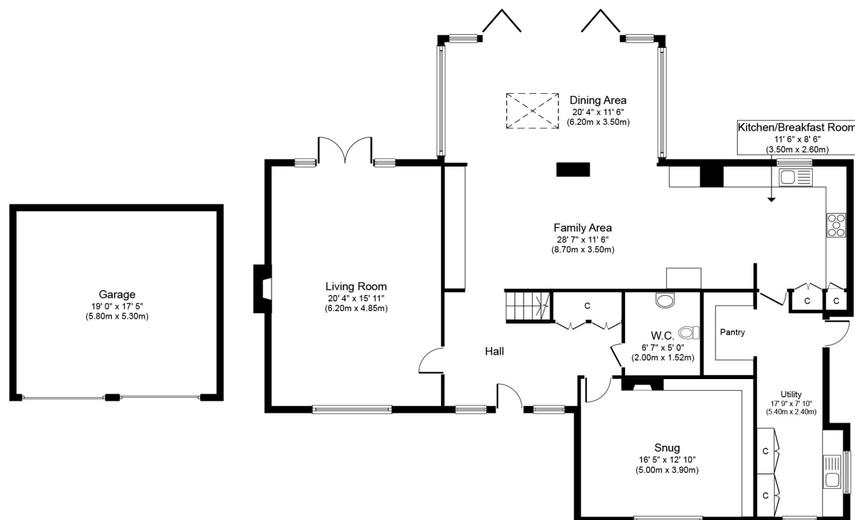
Ground Floor Approximate Floor Area 2054 sq. ft. (190.9 sq. m.)
