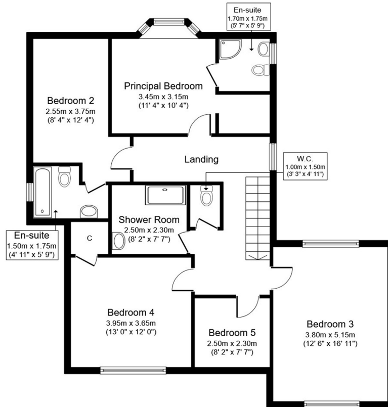
First Floor Approximate Floor Area 1,065 sq. ft. (98.9 sq. m.)
