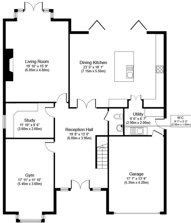
Ground Floor Approximate Floor Area 1,704 sq. ft. (158.4 sq. m.)
