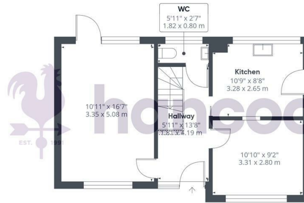
Floor 0
