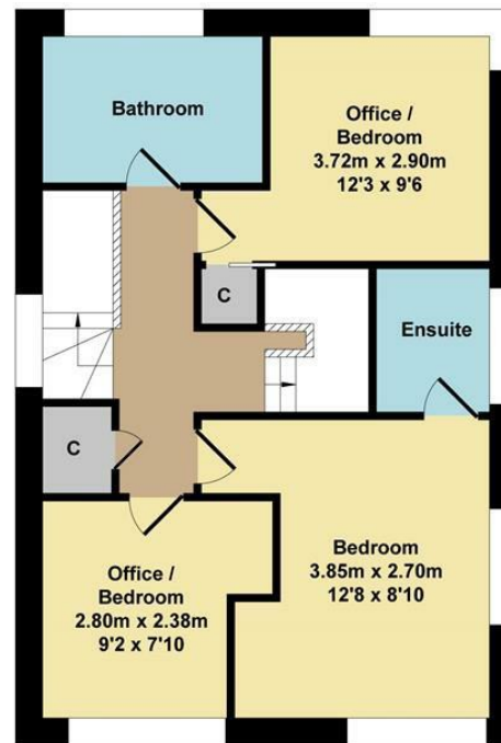
First Floor Approx. Floor Area 50.8 Sq.M. (547 Sq.Ft.)
