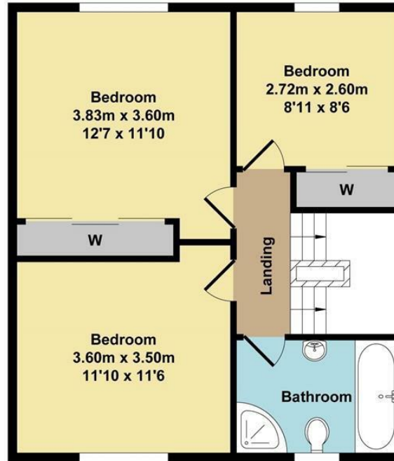
First Floor Approx. Floor Area 47.60 Sq.M. (512 Sq.Ft.)
