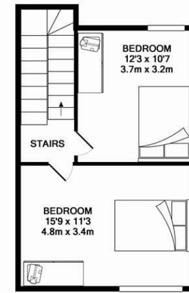
2ND FLOOR APPROX. FLOOR AREA 382 SQ.FT. (35.5 SQ.M.)
