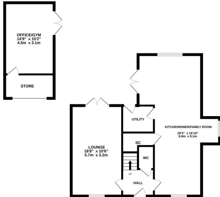
GROUND FLOOR 863 sq.ft. (80.2 sq.m.) approx.
