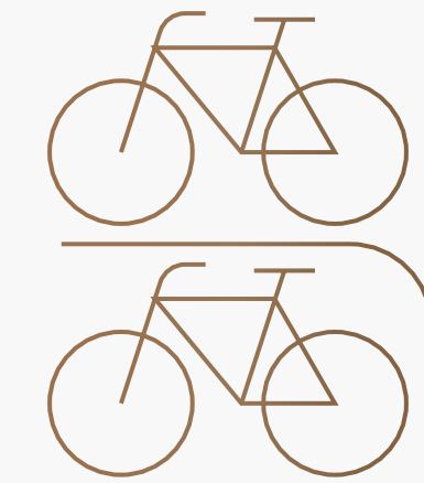
56 bike racks
