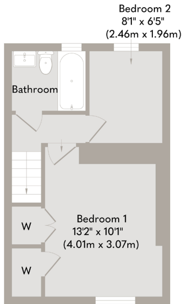
First Floor Approximate Floor Area 286 sq. ft (26.56 sq. m)
