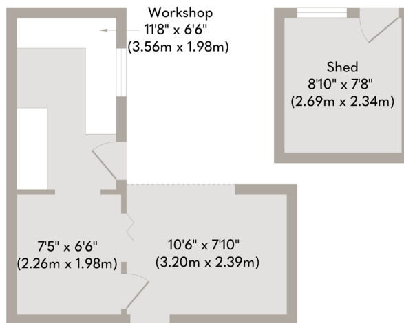
Outbuilding Approximate Floor Area 281 sq. ft (26.14 sq. m)
