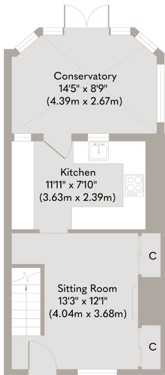
Ground Floor Approximate Floor Area 373 sq. ft (34.67 sq. m)
