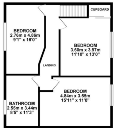
1ST FLOOR 61.21 sq. m. ( 658.87 sq. ft. )
