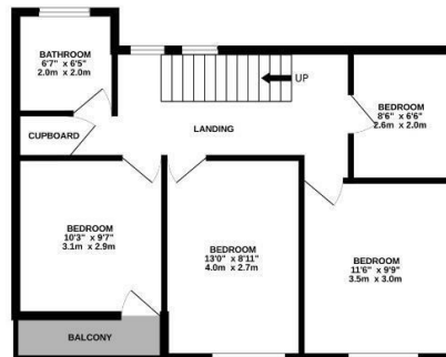
1ST FLOOR 553 sq.ft. (51.4 sq.m.) approx.
