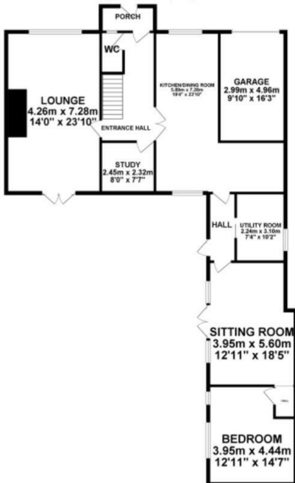
GROUND FLOOR 143.91 sq. m. ( 1549.00 sq. ft. )
