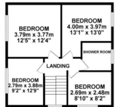
1ST FLOOR 53.13 sq. m. ( 571.93 sq. ft. )
