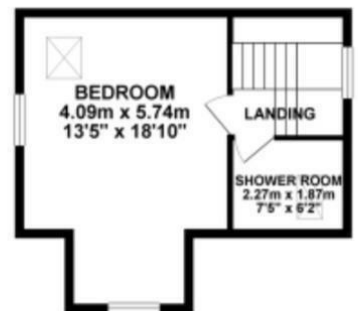
2ND FLOOR 30.64 sq. m. ( 329.83 sq. ft. )
