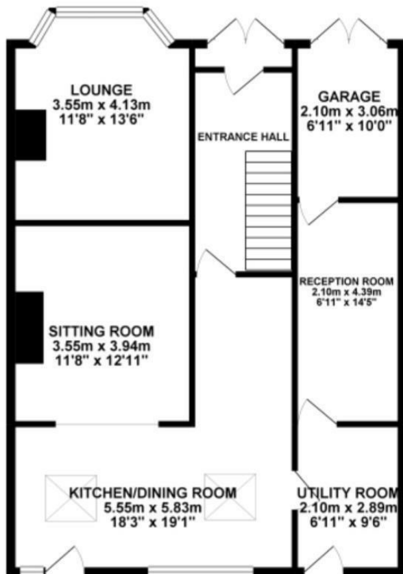
GROUND FLOOR 80.56 sq. m. ( 867.16 sq. ft. )
