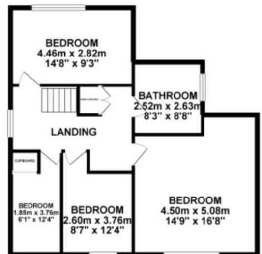
1ST FLOOR 67.69 sq. m. ( 728.63 sq. ft. )
