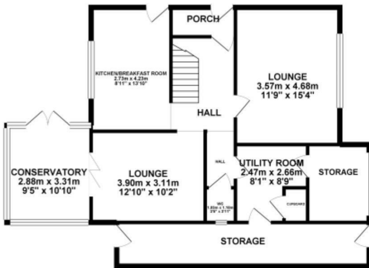
GROUND FLOOR 87.50 sq. m. ( 941.84 sq. ft. )
