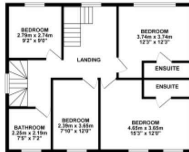
1ST FLOOR 68.74 sq. m. ( 739.91 sq. ft. )
