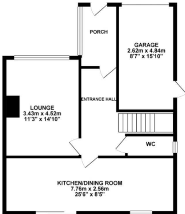
GROUND FLOOR 65.42 sq. m. ( 704.20 sq. ft. )
