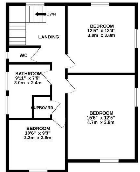
1ST FLOOR 657 sq.ft. (61.0 sq.m.) approx.
