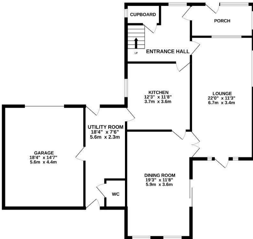
GROUND FLOOR 1207 sq.ft. (112.2 sq.m.) approx.
