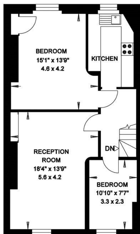
FOURTH FLOOR
