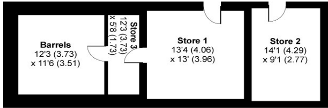
OUTBUILDING GROUND FLOOR
