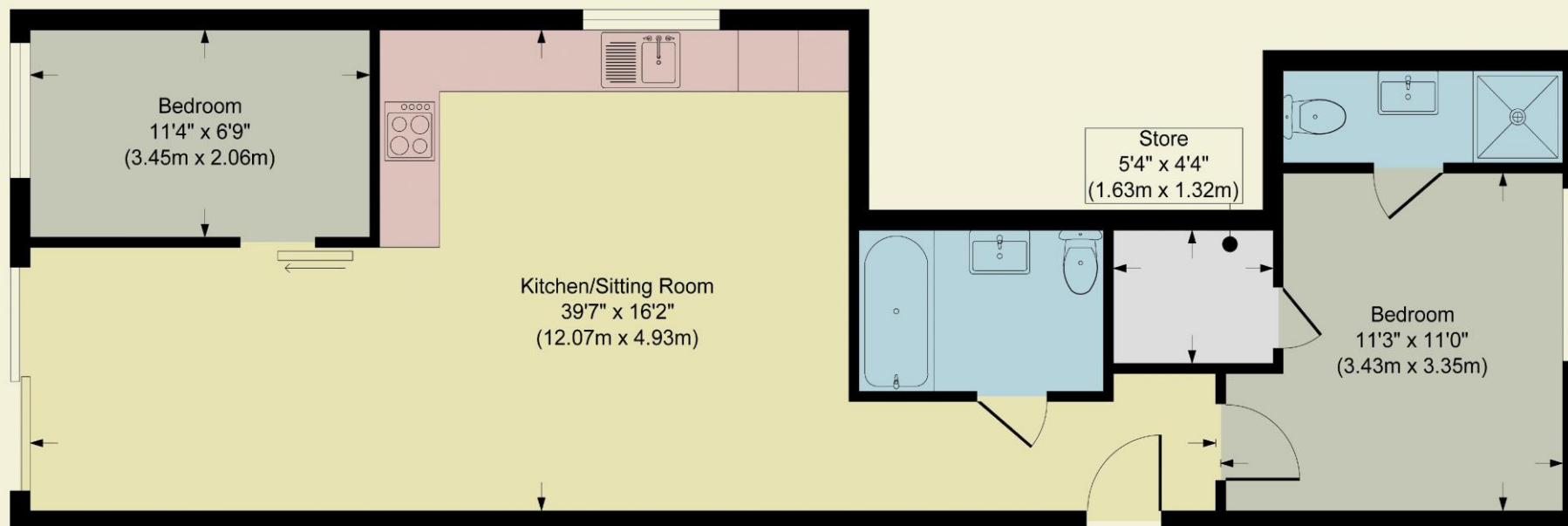
FLAT 1
