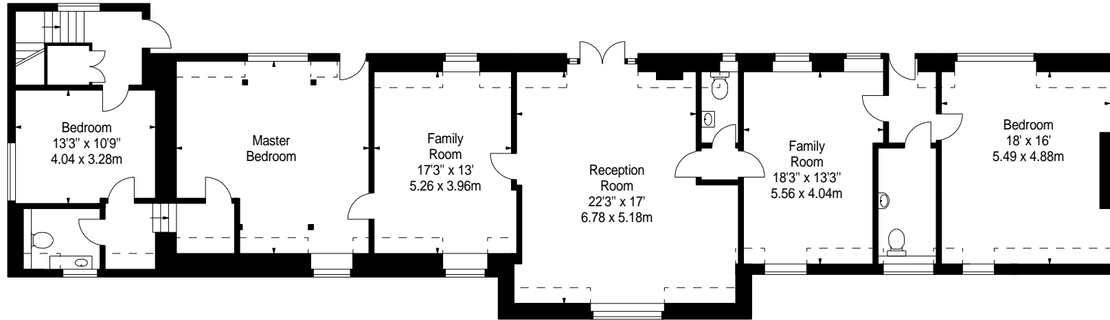
FIRST FLOOR
