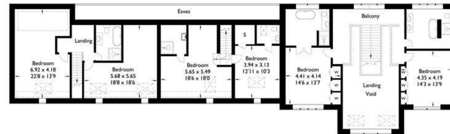
First Floor
