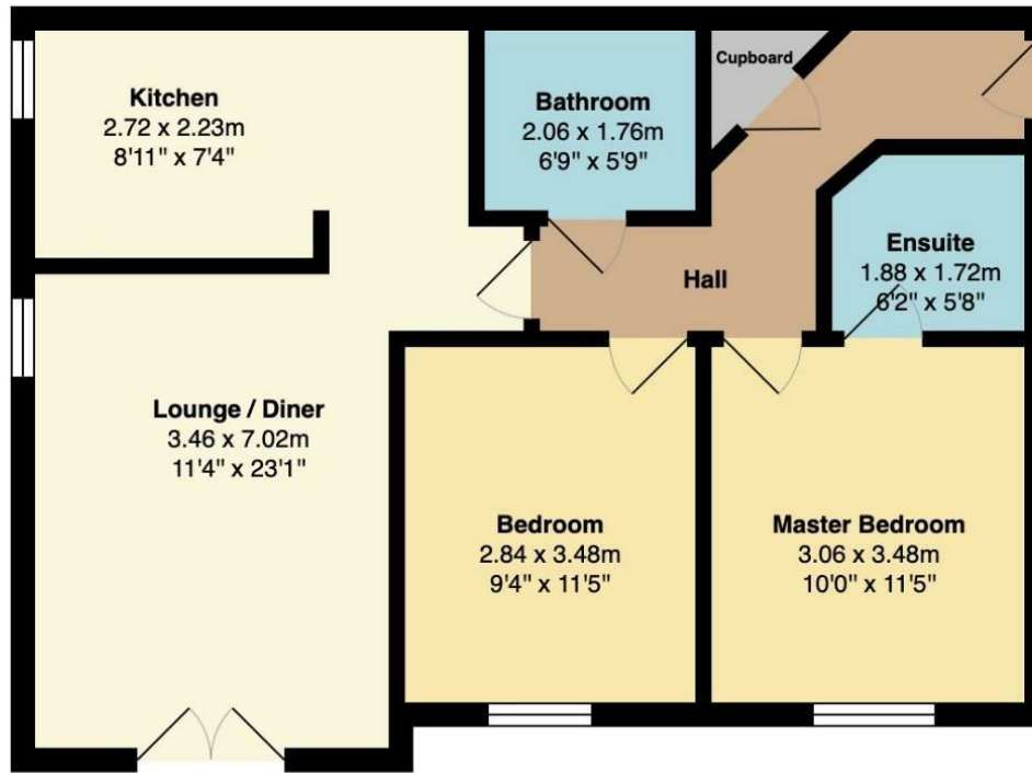
Ground Floor Area: 65.2 m 2 ... 702 ft 2
